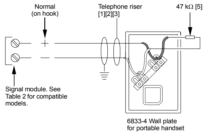
Figure 1: Portable telephone wall plate receptacle wired for three-state operation. Notice that the riser polarity for three-state operation differs from that shown in Figure 2.
