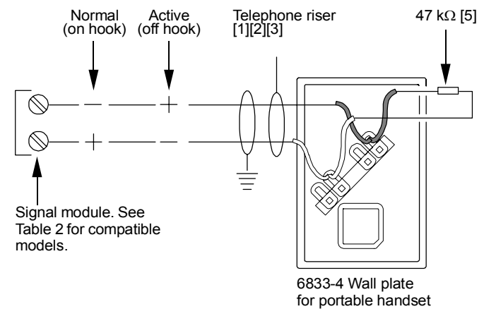
Figure 2: Portable telephone wall plate receptacle wired for four-state operation. Notice that the riser polarity for four-state operation differs from that shown in Figure 1.
